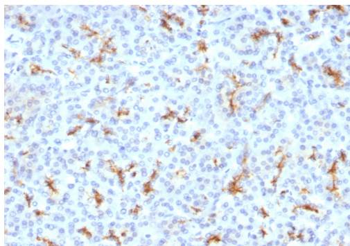
Formalin-fixed, paraffin-embedded human Pancreas stained with CFTR Monoclonal Antibody (CFTR/1342).
