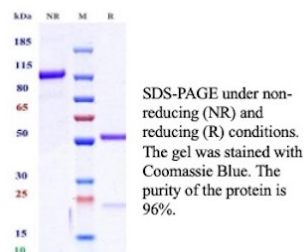
Purity: SDS-PAGE
