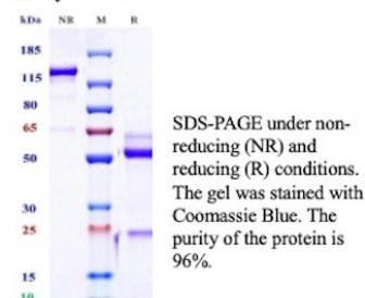
Purity: SDS-PAGE
