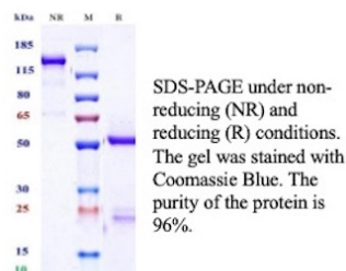
Purity: SDS-PAGE
