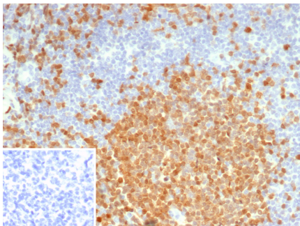
Formalin-fixed, paraffin-embedded human tonsil stained with BOB1 Mouse Monoclonal Antibody (BOB1/2425). Inset: PBS instead of primary antibody; secondary only negative control.
