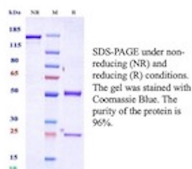
Purity: SDS-PAGE
