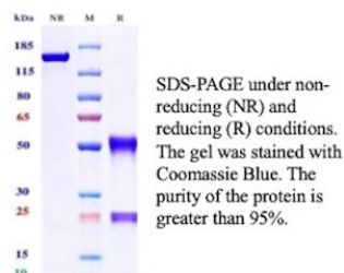
Purity: SDS-PAGE
