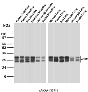
Western Blot Analysis of Intestine and Lung tissue lysates of different species using Annexin A1 Recombinant Mouse Monoclonal Antibody (rANXA1/13711).
