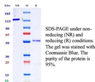
SDS-PAGE Analysis of Purified Annexin A1 Recombinant Mouse Monoclonal Antibody (rANXA1/13711). Confirmation of Purity and Integrity of Antibody.
