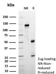
SDS-PAGE Analysis of Purified HLA-E Mouse Monoclonal Antibody (HLAE/13125). Confirmation of Purity and Integrity of Antibody.
