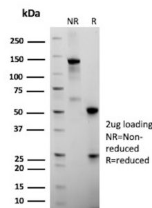
SDS-PAGE Analysis of Purified Folate Receptor Alpha Recombinant Rabbit Monoclonal Antibody (FOLR1/12910R). Confirmation of Purity and Integrity of Antibody.
