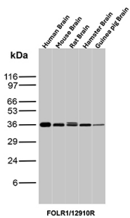
Western Blot Analysis of Human Brain, Mouse Brain, Rat Brain, Hamster Brain and Guinea pig Brain tissue lysates using Folate Receptor alpha Recombinant Rabbit Monoclonal Antibody (FOLR1/12910R).
