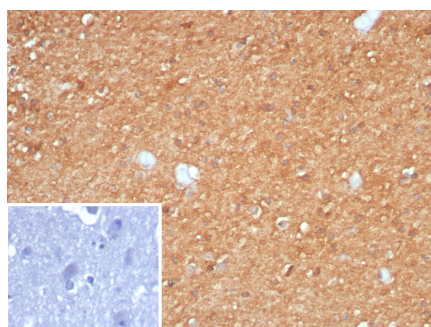
Formalin-fixed, paraffin-embedded human brain stained with CKBB Recombinant Rabbit Monoclonal Antibody (CKBB/8295R). Inset: PBS instead of primary antibody; secondary only negative control.
