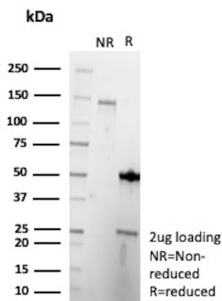
SDS-PAGE Analysis Purified IL7 Recombinant Rabbit Monoclonal Antibody (IL7/13238R). Confirmation of Purity and Integrity of Antibody.
