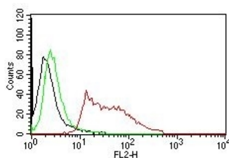
Flow Cytometric analysis of Human Nuclear Antigen on HeLa cells. Black: cells alone; Green: Isotype Control; Red: PE-labeled HNA Monoclonal Antibody (235-1).
