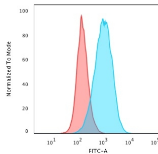
Flow Cytometric Analysis of PFA-fixed Raji cells using CD45RB Mouse Monoclonal Antibody (BRA-11) followed by Goat anti-Mouse-IgG-CF488 (Blue); Isotype Control (Red).
