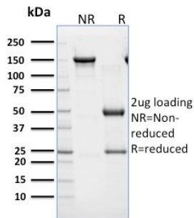
SDS-PAGE Analysis of Purified CD45RB Mouse Monoclonal Antibody (BRA-11). Confirmation of Integrity and Purity of Antibody.
