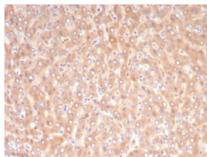
Formalin-fixed, paraffin-embedded human liver stained with ADH1L1 Mouse Monoclonal Antibody (ALDH1L1/7968). HIER: Tris/EDTA, pH9.0, 45min. 2°C: HRP-polymer, 30min. DAB, 5min.
