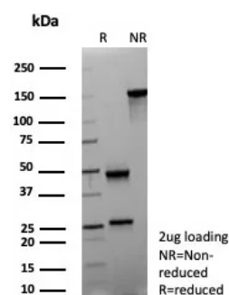
SDS-PAGE Analysis of Purified ADH1L1 Mouse Monoclonal Antibody (ALDH1L1/7968). Confirmation of Purity and Integrity of Antibody.
