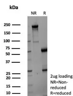
SDS-PAGE Analysis of Purified NSE gamma Mouse Monoclonal Antibody (ENO2/9046). Confirmation of Purity and Integrity of Antibody.
