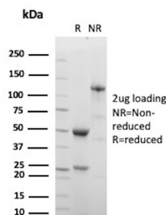
SDS-PAGE Analysis of Purified Myeloperoxidase | Myeloperoxidase | 89 kDa myeloperoxidase | 84 kDa myeloperoxidase | Myeloperoxidase light chain | Myeloperoxidase heavy chain Recombinant Rabbit Monoclonal Antibody (MPO/8997R). Confirmation of Purity and Integrity of Antibody.
