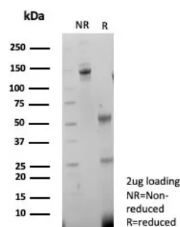
SDS-PAGE Analysis of Purified CD56 Recombinant Mouse Monoclonal Antibody (rNCAM1/8758). Confirmation of Purity and Integrity of Antibody.
