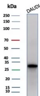
Western blot analysis of Daudi cell lysate using Haptoglobin (HP) Mouse Monoclonal Antibody (HP/3834).
