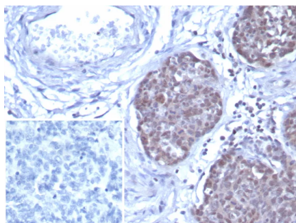
Formalin-fixed, paraffin-embedded human ovarian cancer stained with GATA-3 Recombinant Rabbit Monoclonal Antibody (GATA3/7686R). Inset: PBS instead of primary antibody; secondary only negative control.
