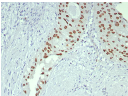
Formalin-fixed, paraffin-embedded human bladder stained with GATA-3 Recombinant Rabbit Monoclonal Antibody (GATA3/7686R). HIER: Tris/EDTA, pH9.0, 45min. 2°C: HRP-polymer, 30min. DAB, 5min.
