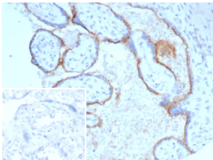
Formalin-fixed, paraffin-embedded human placenta stained with Endoglin / CD105 Recombinant Rabbit Monoclonal Antibody (ENG/8069R) Inset: PBS instead of primary antibody; secondary only negative control.
