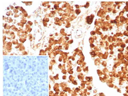
Formalin-fixed, paraffin-embedded human pancreas stained with CPA1 Recombinant Rabbit Monoclonal Antibody (CPA1/8624R). Inset: PBS instead of primary antibody; secondary only negative control.
