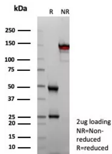
SDS-PAGE Analysis of Purified CPA1 Recombinant Rabbit Monoclonal Antibody (CPA1/8624R). Confirmation of Purity and Integrity of Antibody.
