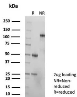
SDS-PAGE Analysis of Purified TAG-72 Rabbit Recombinant Monoclonal Antibody (TAG72/8317R). Confirmation of Purity and Integrity of Antibody.
