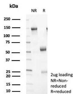
SDS-PAGE Analysis of Purified 14-3-3E Recombinant Rabbit Monoclonal Antibody (YWHAE/8309R). Confirmation of Purity and Integrity of Antibody.
