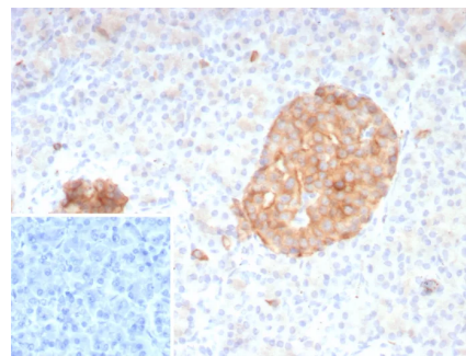
Formalin-fixed, paraffin-embedded human pancreas stained with Synaptophysin Recombinant Mouse Monoclonal Antibody (rSYP/8807). Inset: PBS instead of primary antibody; secondary only negative control.
