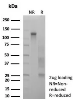
SDS-PAGE Analysis of Purified Synaptophysin Recombinant Mouse Monoclonal Antibody (rSYP/8807). Confirmation of Purity and Integrity of Antibody.
