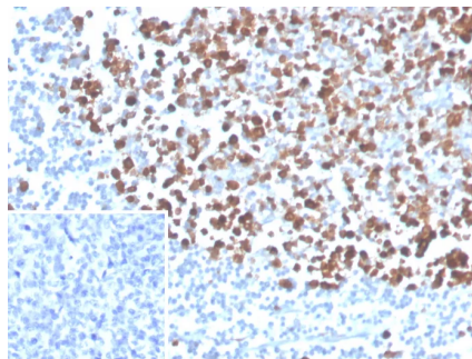
Formalin-fixed, paraffin-embedded human tonsil stained with PCNA Mouse Monoclonal Antibody (PCNA/4540) at 2ug/ml. Inset: PBS instead of primary antibody; secondary only negative control.
