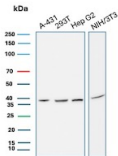
Western Blot Analysis of A-431, 293T, Hep G2 and NIH/3T3 cell lysates using PCNA Mouse Monoclonal Antibody (PCNA/4540).
