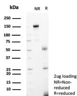
SDS-PAGE Analysis of Purified PCNA Mouse Monoclonal Antibody (PCNA/4540). Confirmation of Purity and Integrity of Antibody.
