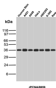
Western Blot Analysis of Human Skin, A431, A549, HeLa, HEK293, K-562 and Raw lysates using PCNA Recombinant Mouse Monoclonal Antibody (rPCNA/8859).
