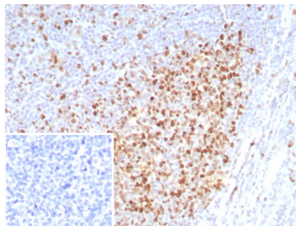
Formalin-fixed, paraffin-embedded human tonsil stained with PCNA Recombinant Mouse Monoclonal Antibody (rPCNA/8859) at 2ug/ml. Inset: PBS instead of primary antibody; secondary only negative control.
