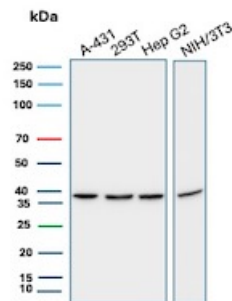
Western Blot Analysis of A-431, 293T, Hep G2 and NIH/3T3 cell lysates using PCNA Recombinant Mouse Monoclonal Antibody (rPCNA/8859).
