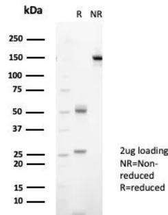
SDS-PAGE Analysis of Purified NME2 / nm23-H2 Mouse Monoclonal Antibody (NME2/6434). Confirmation of Purity and Integrity of Antibody.
