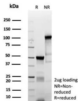
SDS-PAGE Analysis of Purified MyoD1 Recombinant Rabbit Monoclonal Antibody (MYOD1/9405R). Confirmation of Purity and Integrity of Antibody.
