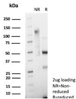
SDS-PAGE Analysis of Purified SYP Recombinant Rabbit Monoclonal Antibody (SYP/7976R). Confirmation of Purity and Integrity of Antibody.
