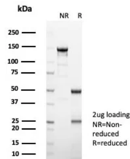
SDS-PAGE Analysis of Purified Interleukin-2 (IL-2) Mouse Monoclonal Antibody (IL2/4988). Confirmation of Purity and Integrity of Antibody.
