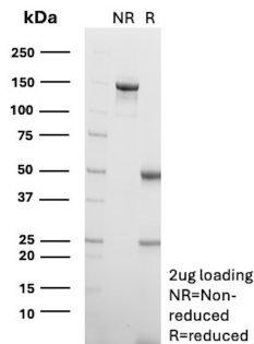
SDS-PAGE Analysis of Purified CD74 Mouse Monoclonal Antibody (CLIP/7946). Confirmation of Purity and Integrity of Antibody.
