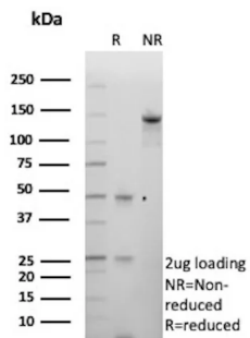
SDS-PAGE Analysis Purified CDH6 Mouse Monoclonal Antibody (CDH6/9347). Confirmation of Purity and Integrity of Antibody.
