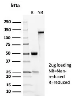
SDS-PAGE Analysis of Purified p53 Recombinant Rabbit Monoclonal Antibody (TP53/7082R). Confirmation of Purity and Integrity of Antibody.
