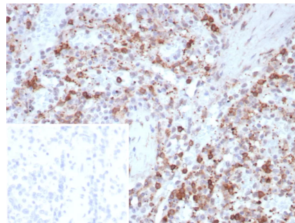
Formalin-fixed, paraffin-embedded human spleen stained with Osteonectin Recombinant Mouse Monoclonal Antibody (rOSTN/8527). Inset: PBS instead of primary antibody; secondary only negative control.
