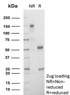
SDS-PAGE Analysis of Purified CD27 Recombinant Rabbit Monoclonal Antibody(LPFS2/8574R). Confirmation of Purity and Integrity of Antibody
