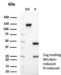
SDS-PAGE Analysis of Purified NSE gamma Mouse Monoclonal Antibody (ENO2/6680). Confirmation of Purity and Integrity of Antibody.
