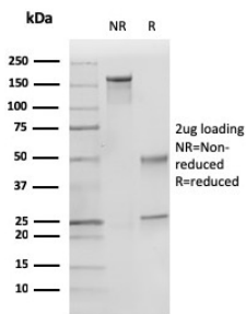
SDS-PAGE Analysis Purified p27 Mouse Monoclonal Antibody (KIP1/769). Confirmation of Purity and Integrity of Antibody.
