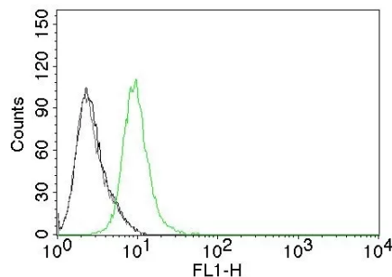
Flow Cytometry of human p27 on Jurkat cells. Black: cells alone; Grey: Isotype Control; Green: CF488-labeled p27 Monoclonal Antibody (KIP1/769).
