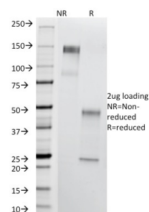
SDS-PAGE Analysis of Purified T-F Antigen Mouse Monoclonal Antibody (A84-A/F10). Confirmation of Purity and Integrity of Antibody.
