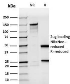
SDS-PAGE Analysis of Purified BrdU Recombinant Mouse Monoclonal Antibody (rBRD494). Confirmation of Purity and Integrity of Antibody.
