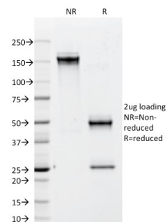
SDS-PAGE Analysis of Purified CD79b Mouse Monoclonal Antibody (IGB/1842). Confirmation of Integrity and Purity of Antibody.
