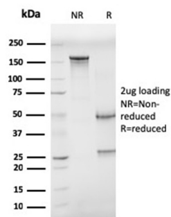
SDS-PAGE Analysis of Purified CD68 Mouse Monoclonal Antibody (CD68/G2). Confirmation of Integrity and Purity of Antibody.
