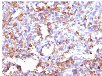
Formalin-fixed, paraffin-embedded human Histiocytoma stained with CD68 Mouse Monoclonal Antibody (CD68/G2).
