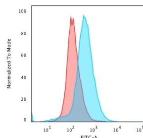
Flow Cytometric Analysis of paraformaldehyde-fixed Jurkat cells using CD28 Mouse Monoclonal Antibody (C28/76) followed by goat anti-Mouse IgG-CF488 (Blue); Isotype control (Red).
