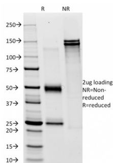
SDS-PAGE Analysis of Purified CD28 Mouse Monoclonal Antibody (C28/76). Confirmation of Integrity and Purity of Antibody.
