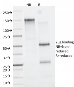
SDS-PAGE Analysis Purified CD163-Monospecific Mouse Monoclonal Antibody (M130/2162). Confirmation of Purity and Integrity of Antibody.
