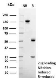
SDS-PAGE Analysis Purified CD14 Mouse Monoclonal Antibody (LPSR/553). Confirmation of Purity and Integrity of Antibody.
