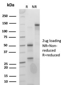
SDS-PAGE Analysis of Purified T-cell surface antigen CD2 Mouse Monoclonal Antibody (LFA2/7106). Confirmation of Purity and Integrity of Antibody.
