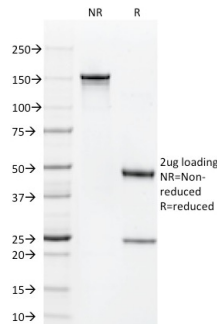
SDS-PAGE Analysis of Purified CD1a Mouse Monoclonal Antibody (C1A/711). Confirmation of Integrity and Purity of Antibody.
