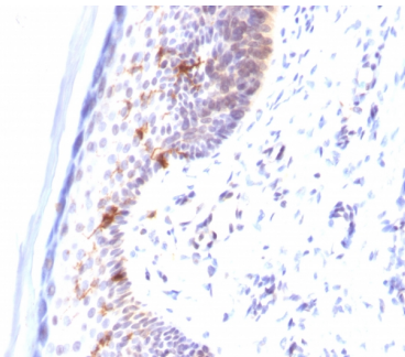
Formalin-fixed, paraffin-embedded human Skin stained with CD1a Mouse Monoclonal Antibody (C1A/711).
