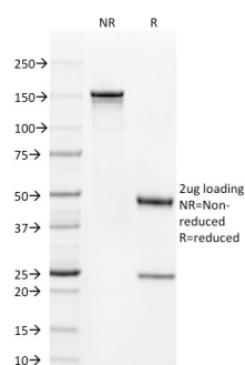
SDS-PAGE Analysis of Purified CD1a Mouse Monoclonal Antibody (O10). Confirmation of Integrity and Purity of Antibody.
