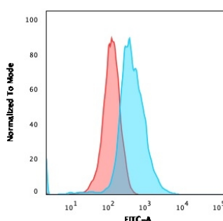
Flow Cytometric Analysis of MOLT-4 cells using CD1a Mouse Monoclonal Antibody (O10) followed by goat anti-Mouse IgG-CF488 (Blue); Isotype control (Red).
