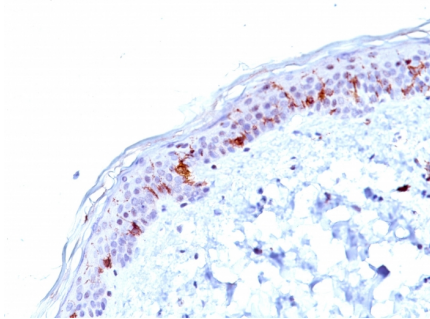
Formalin-fixed, paraffin-embedded human Skin stained with CD1a Mouse Monoclonal Antibody (O10).
