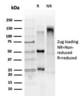
SDS-PAGE Analysis of Purified GTF2IRD2 Mouse Monoclonal Antibody(PCRP-GTF2IRD2-1B4). Confirmation of Purity and Integrity of Antibody.
