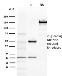
SDS-PAGE Analysis of Purified BAP1 Mouse Monoclonal Antibody (BAP1/2432). Confirmation of Purity and Integrity of Antibody.
